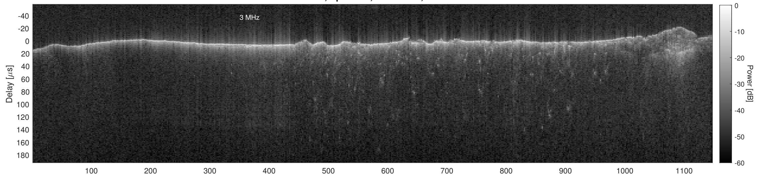
Orbit 15282, Cluttergram
