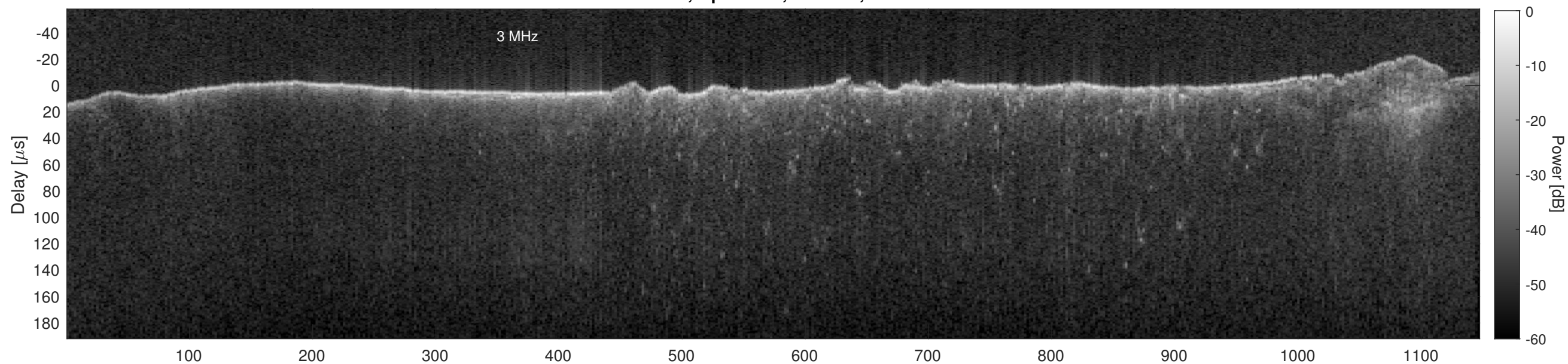
Orbit 15282, Cluttergram
