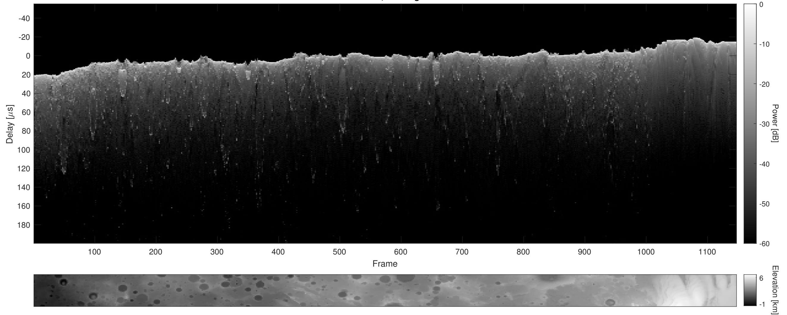
Orbit 15284, Cluttergram
