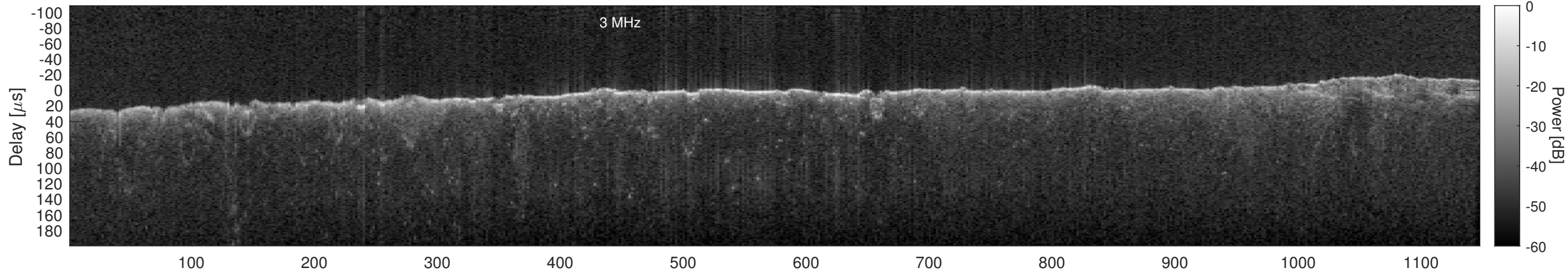
Orbit 15284, Window, Channel 2, Chapman
