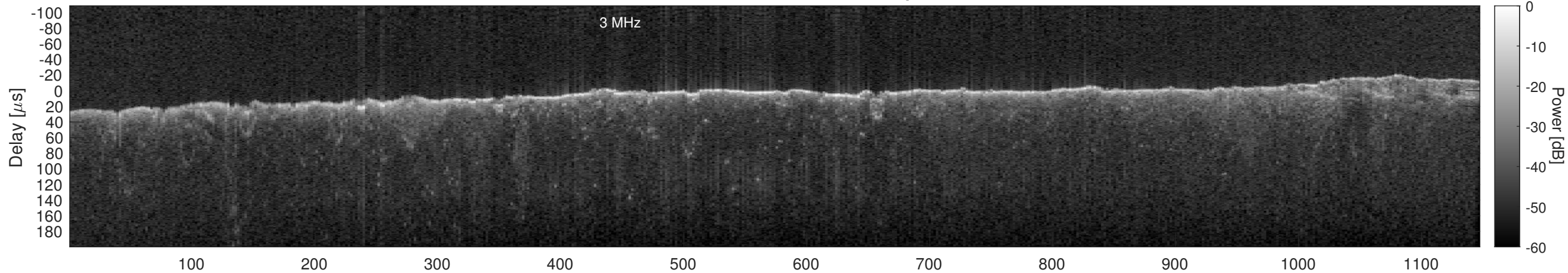
Orbit 15284, Window, Channel 2, Optimized
