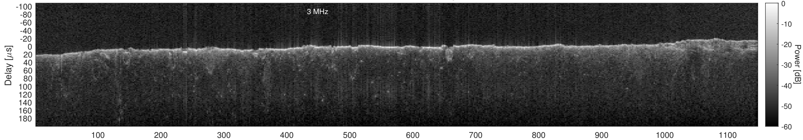
Orbit 15284, Cluttergram
