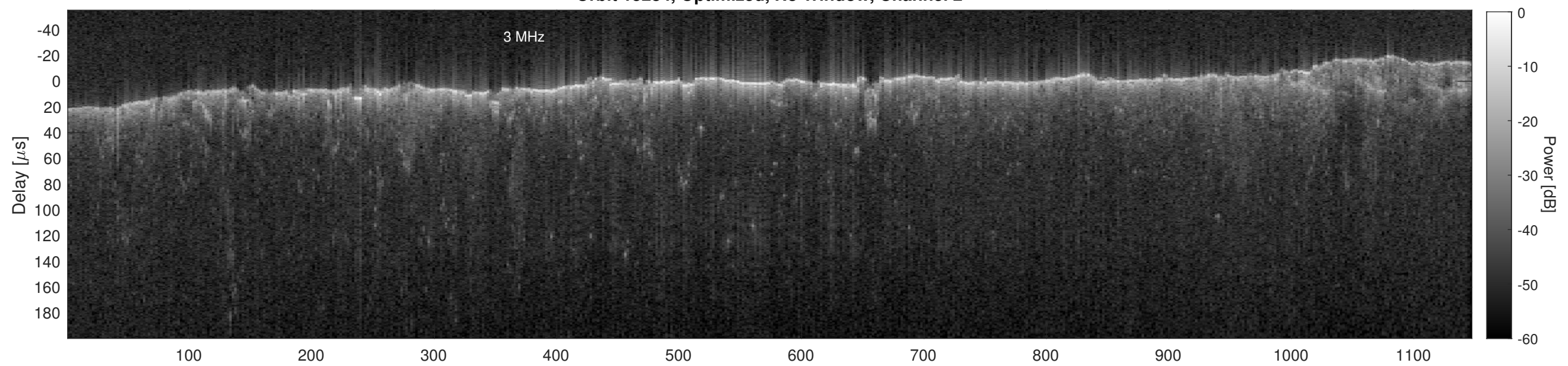
Orbit 15284, Cluttergram
