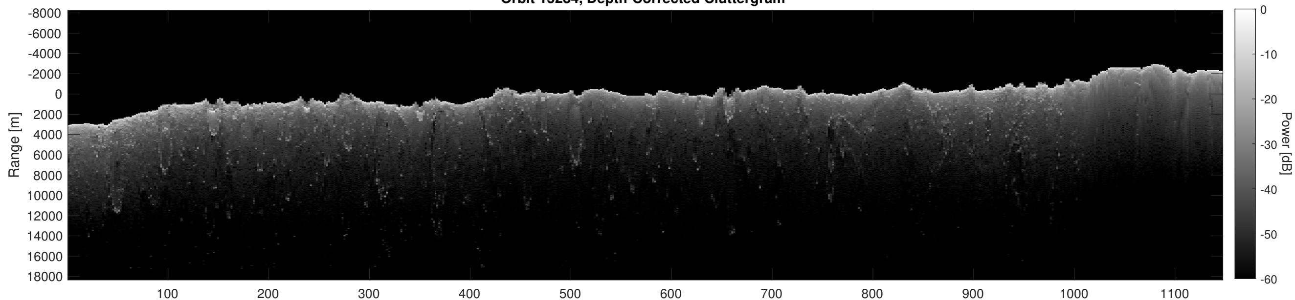
Orbit 15284, Depth-Corrected Cluttergram
