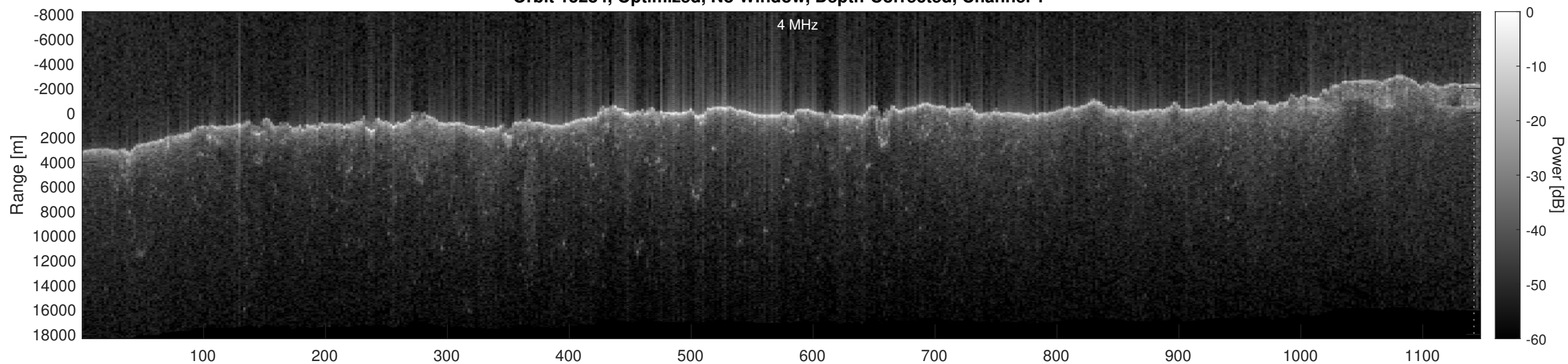
Orbit 15284, Optimized, No Window, Depth-Corrected, Channel 2
