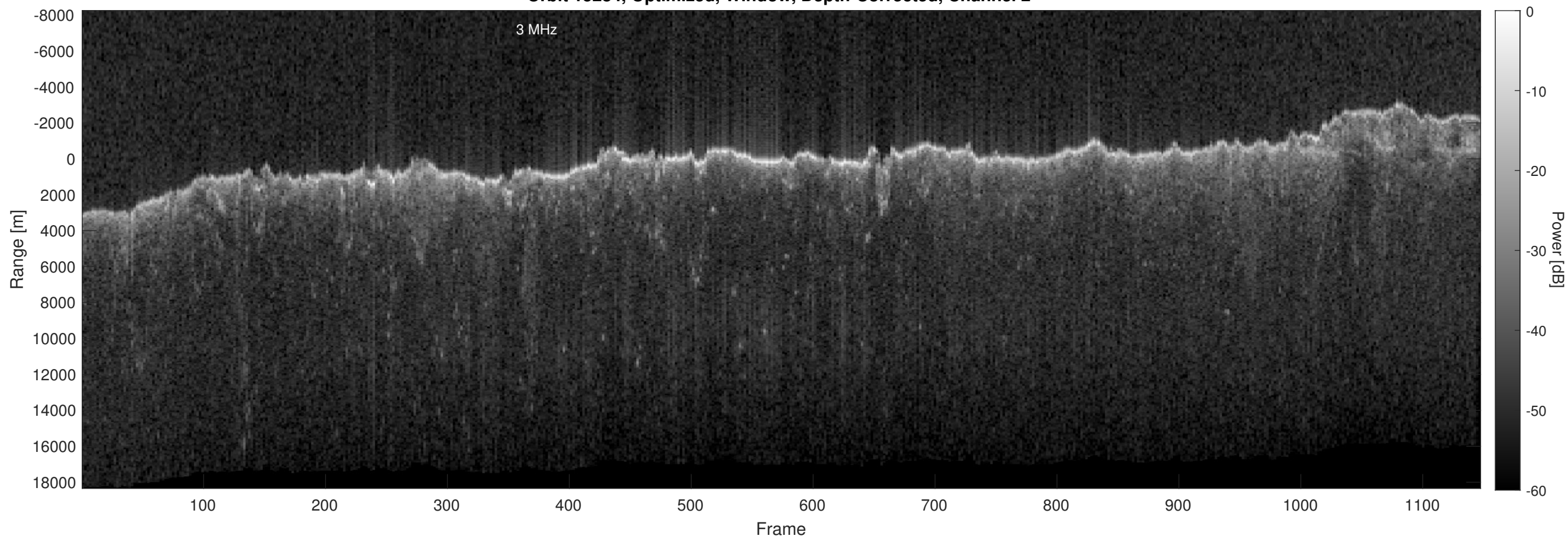
Orbit 15284, Optimized, Window, Depth-Corrected, Channel 2
