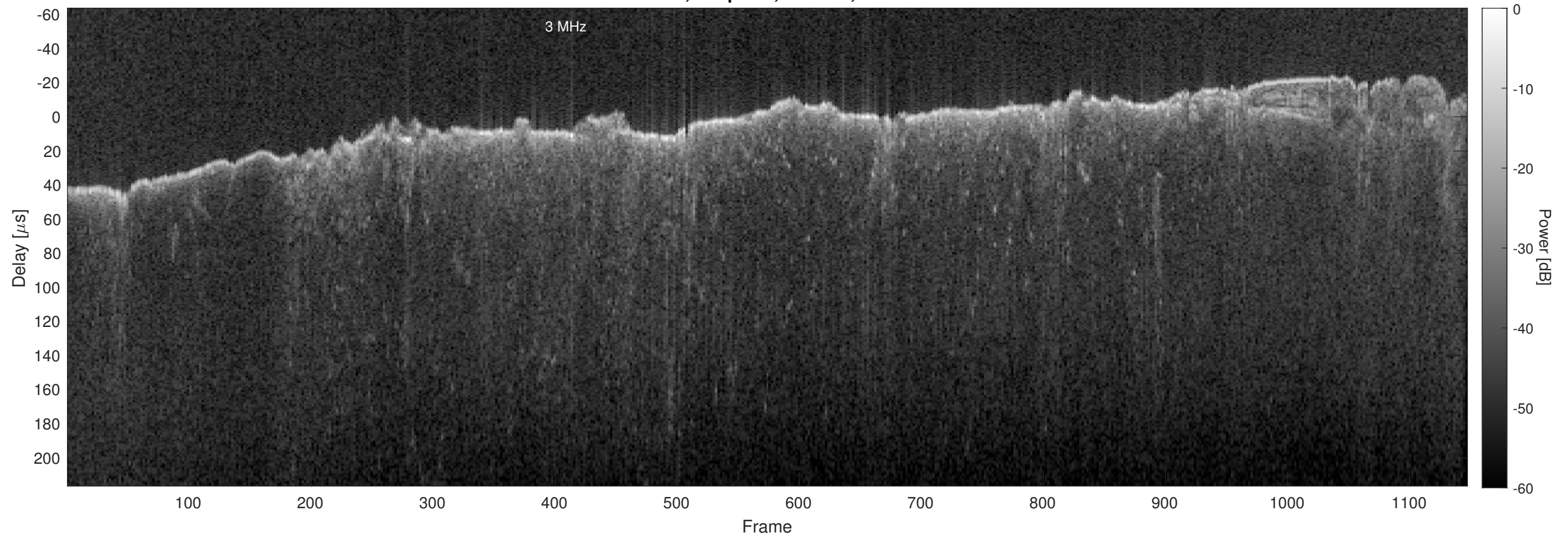
Orbit 15286, Chapman, Window, Channel 2
