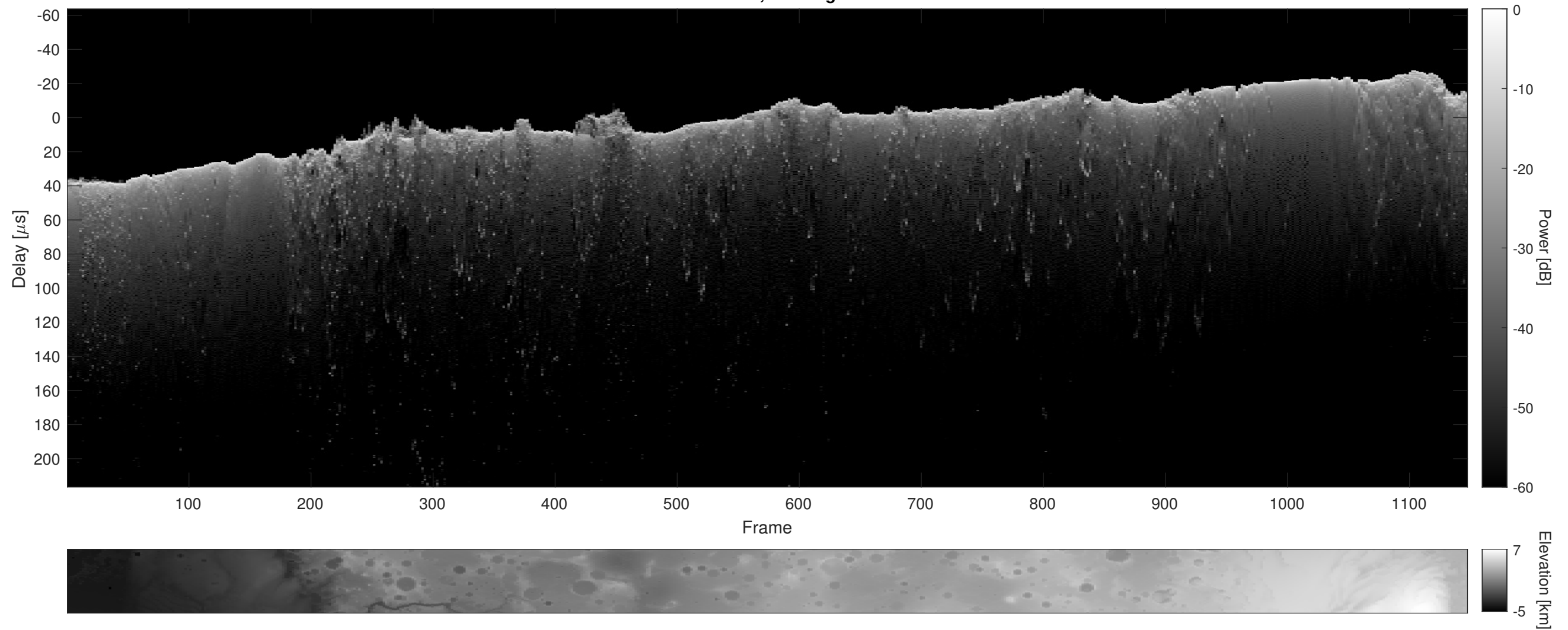
Orbit 15286, Cluttergram
