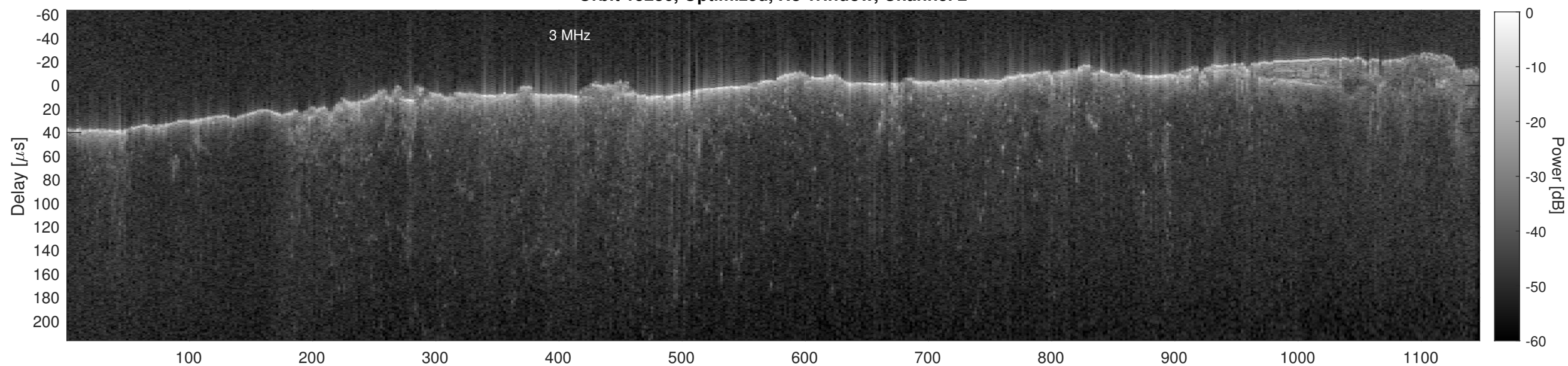
Orbit 15286, Cluttergram
