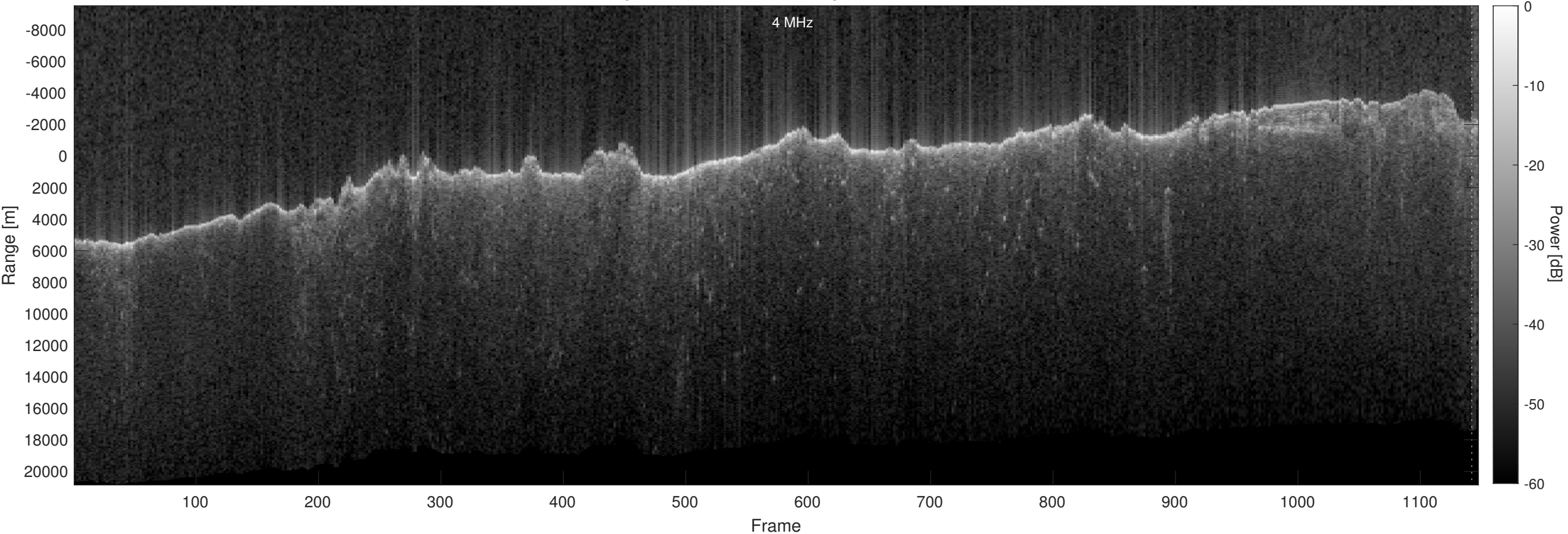
Orbit 15286, Optimized, No Window, Depth-Corrected, Channel 2
