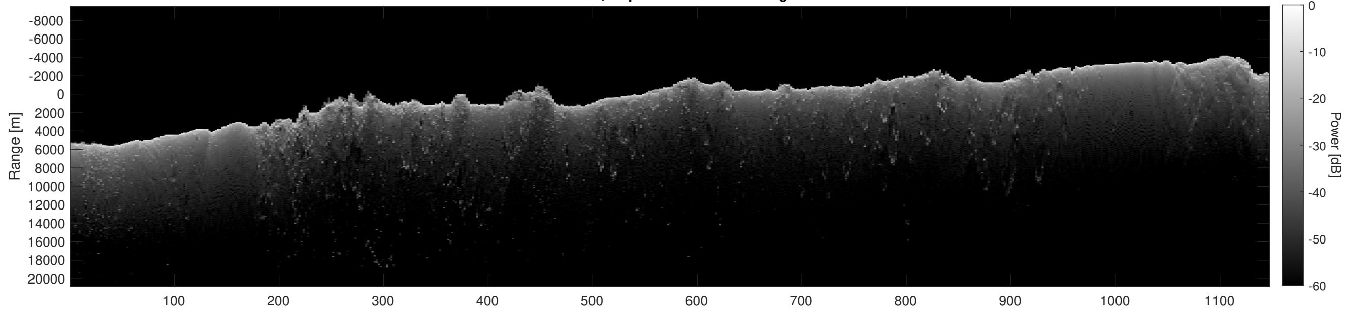
Orbit 15286, Depth-Corrected Cluttergram
