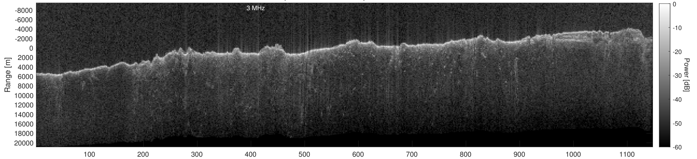
Orbit 15286, Depth-Corrected Cluttergram
