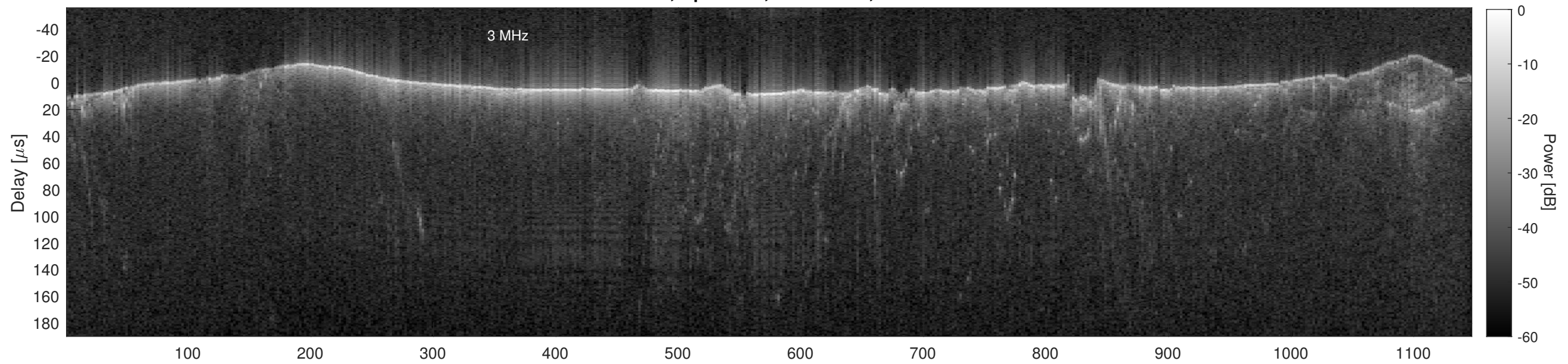
Orbit 15289, Cluttergram
