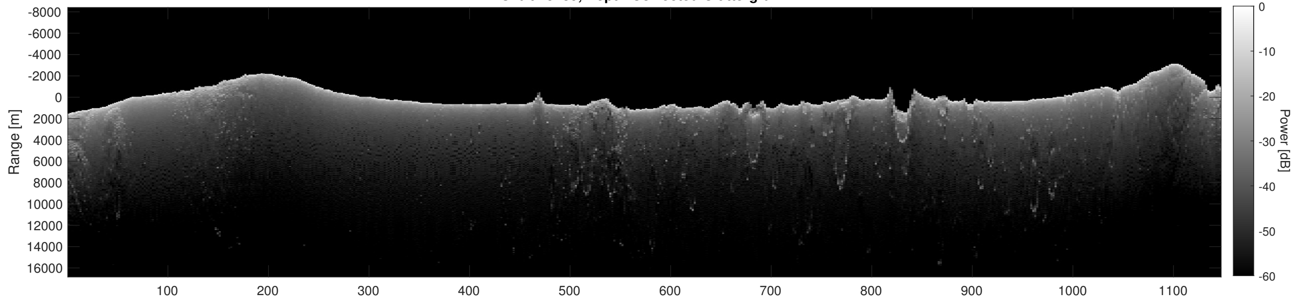
Orbit 15289, Depth-Corrected Cluttergram
