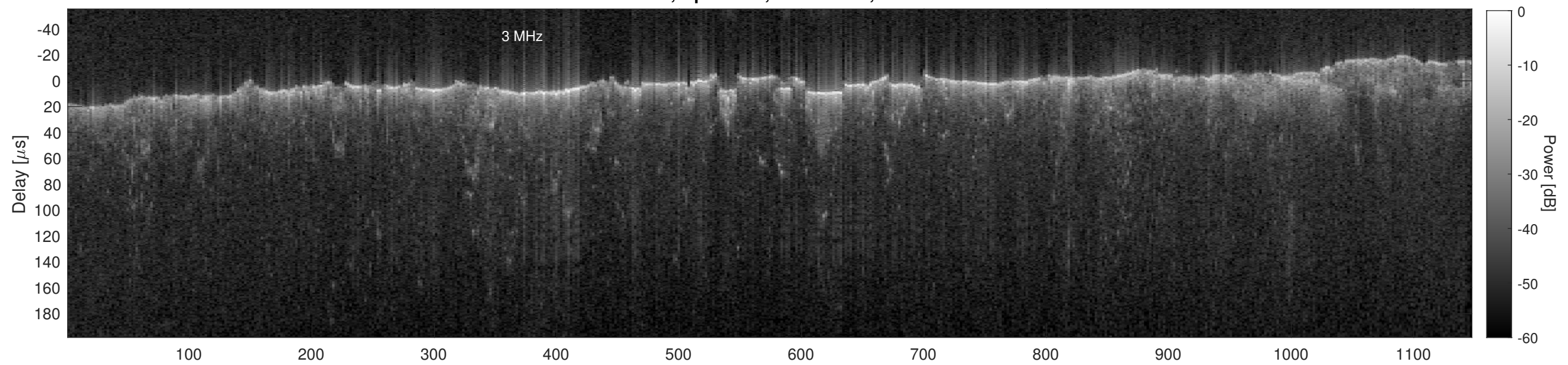
Orbit 15291, Cluttergram
