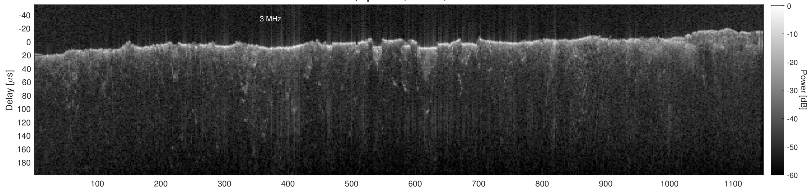
Orbit 15291, Cluttergram
