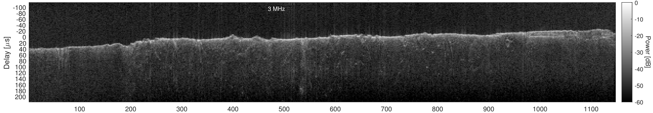
Orbit 15293, Cluttergram
