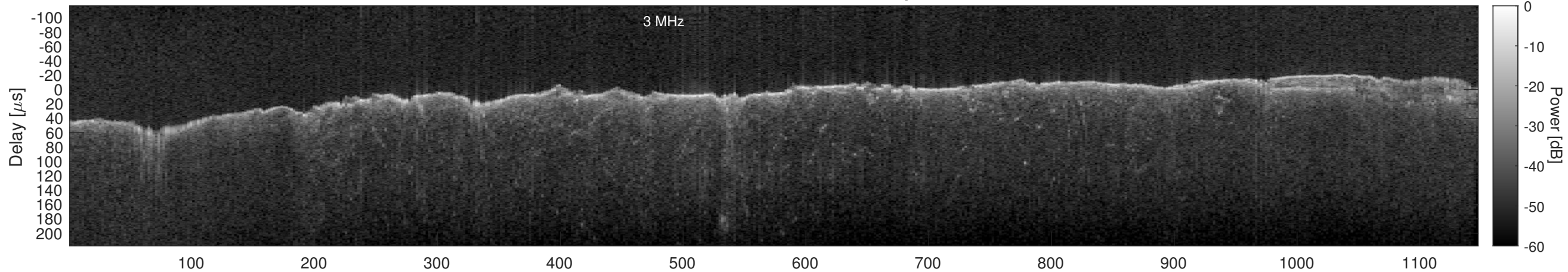
Orbit 15293, Window, Channel 2, Optimized
