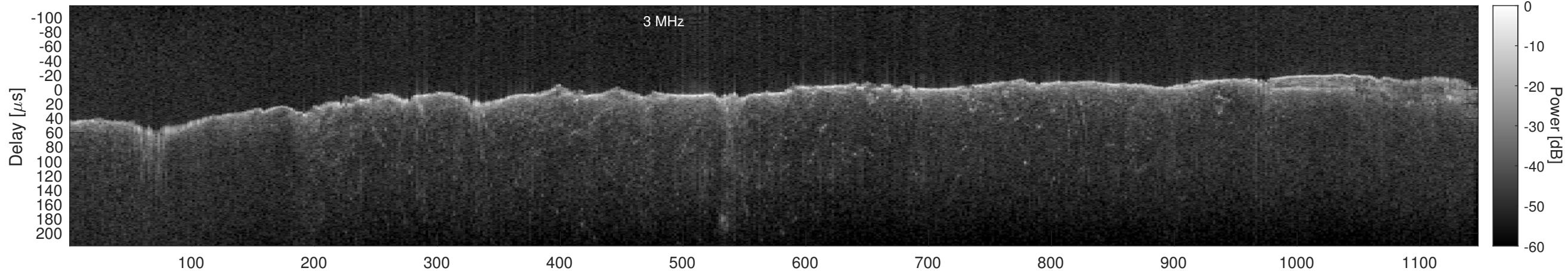
Orbit 15293, Window, Channel 2, Chapman
