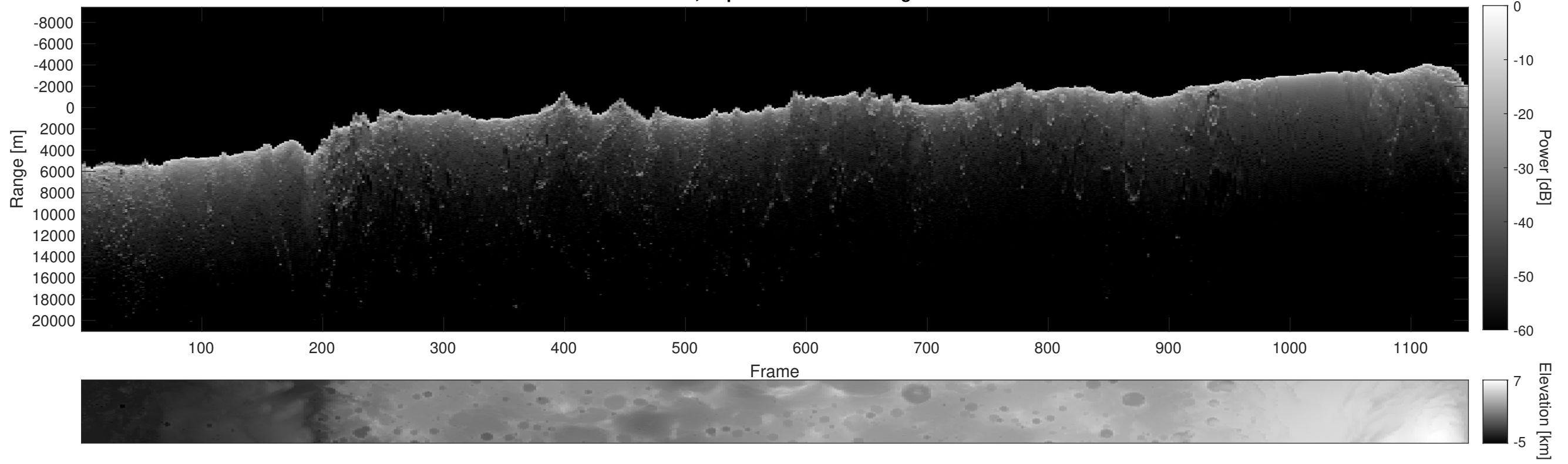
Orbit 15293, Depth-Corrected Cluttergram
