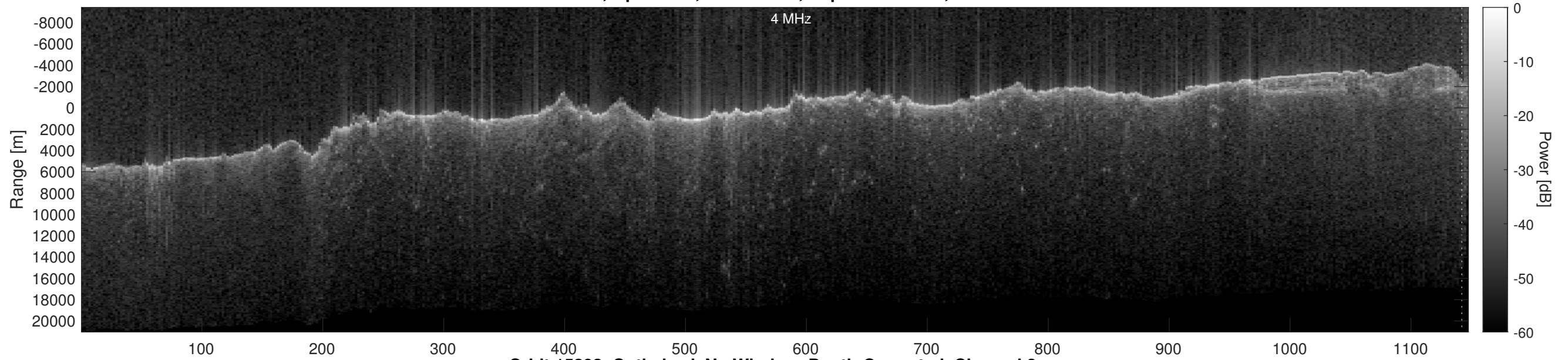
Orbit 15293, Optimized, No Window, Depth-Corrected, Channel 2
