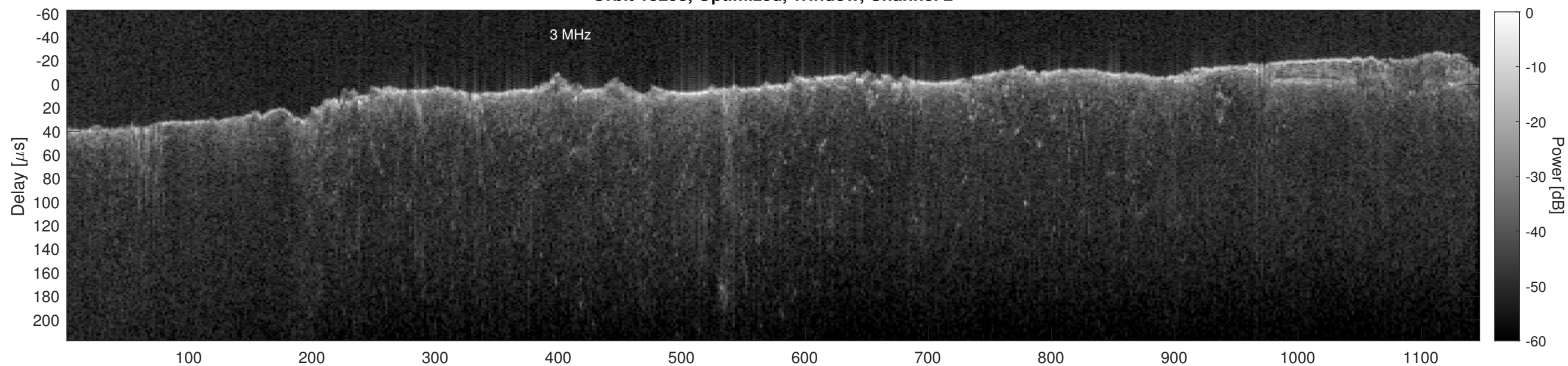
Orbit 15293, Cluttergram
