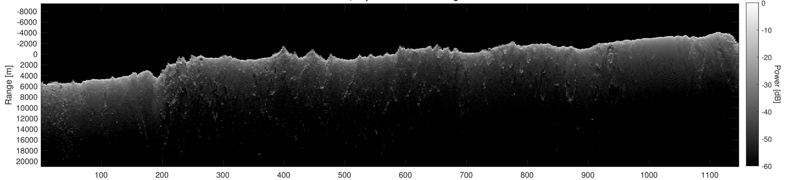
Orbit 15293, Depth-Corrected Cluttergram
