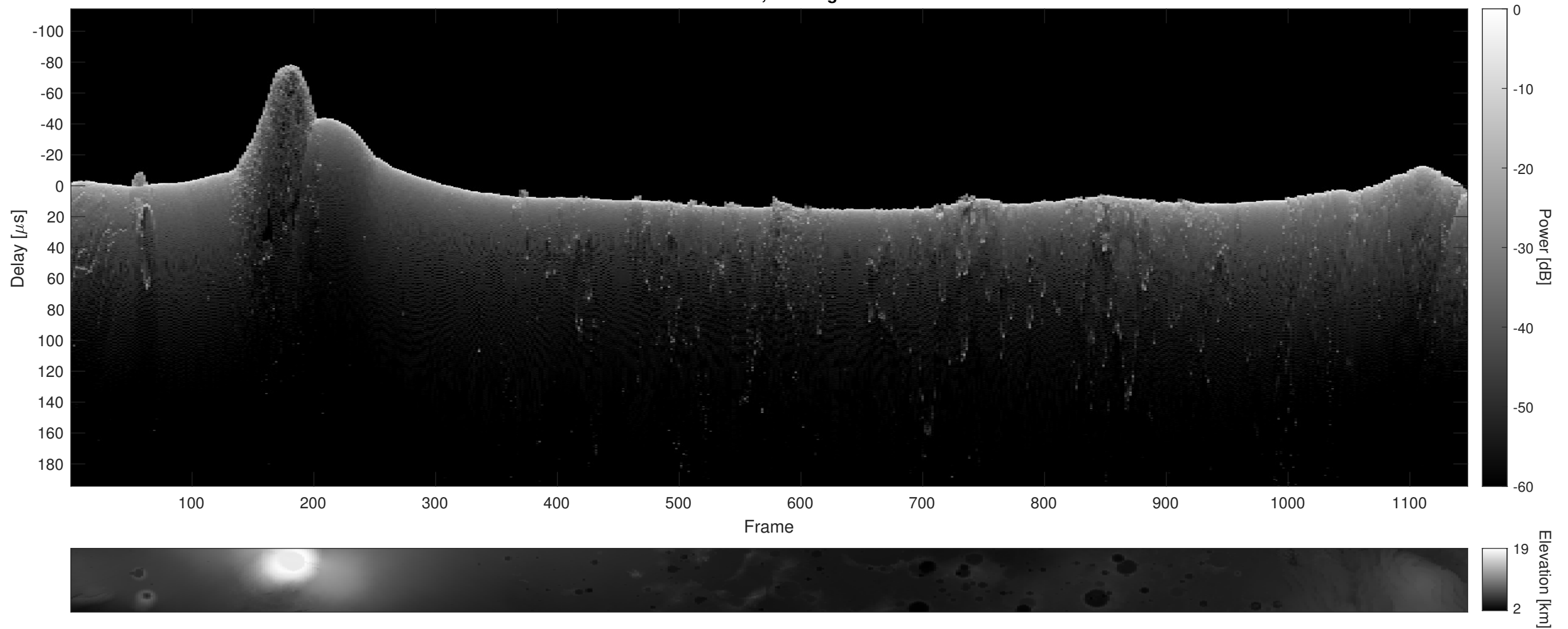
Orbit 15296, Cluttergram
