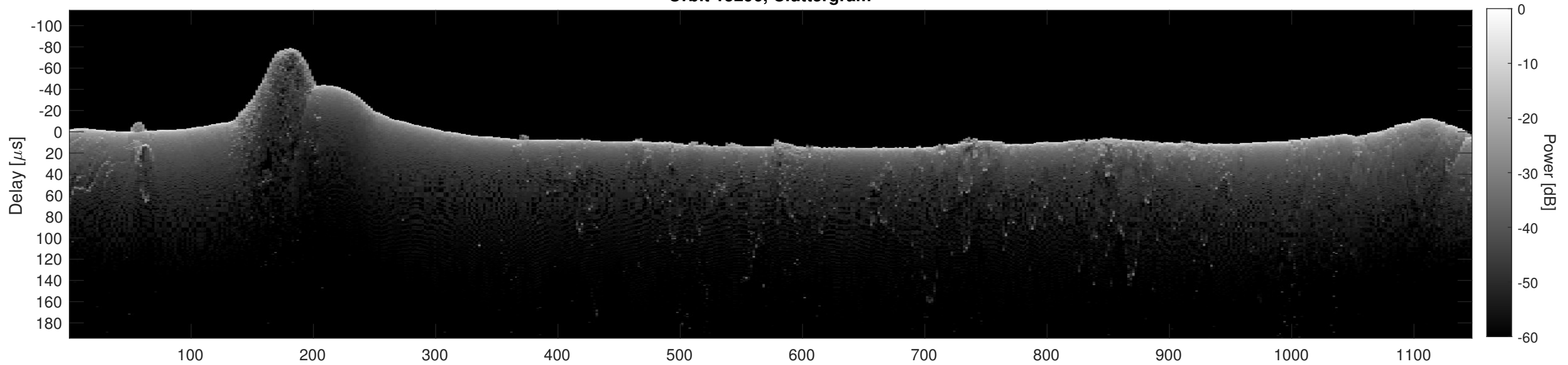
Orbit 15296, Cluttergram
