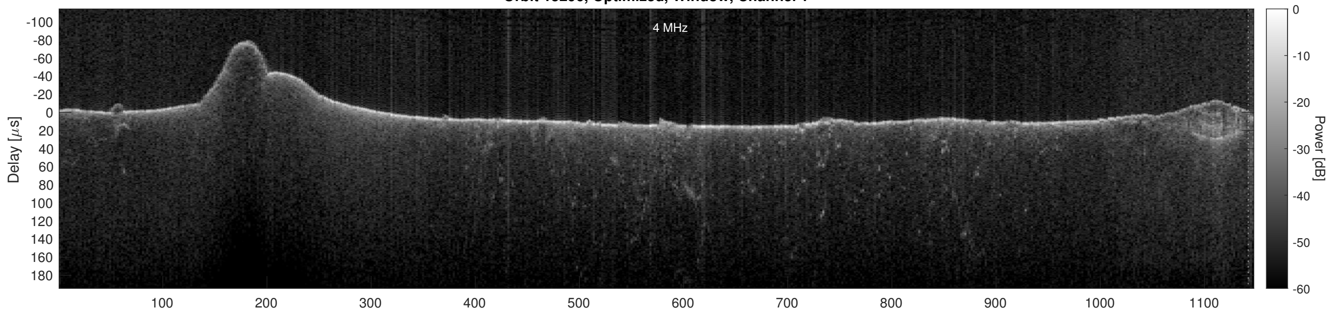
Orbit 15296, Optimized, Window, Channel 2
