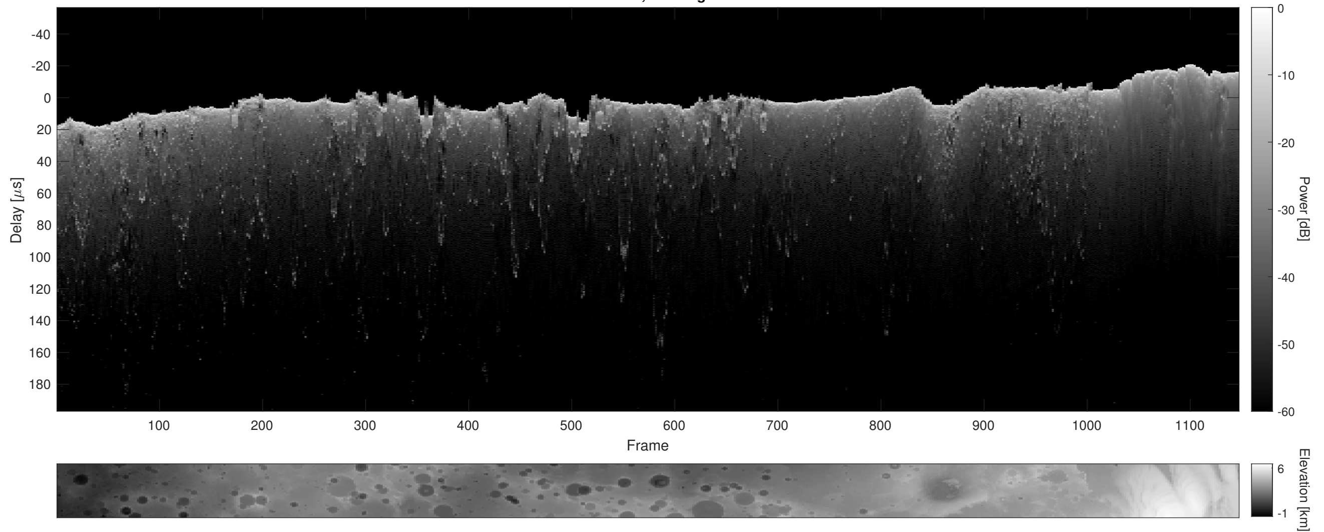
Orbit 15298, Cluttergram
