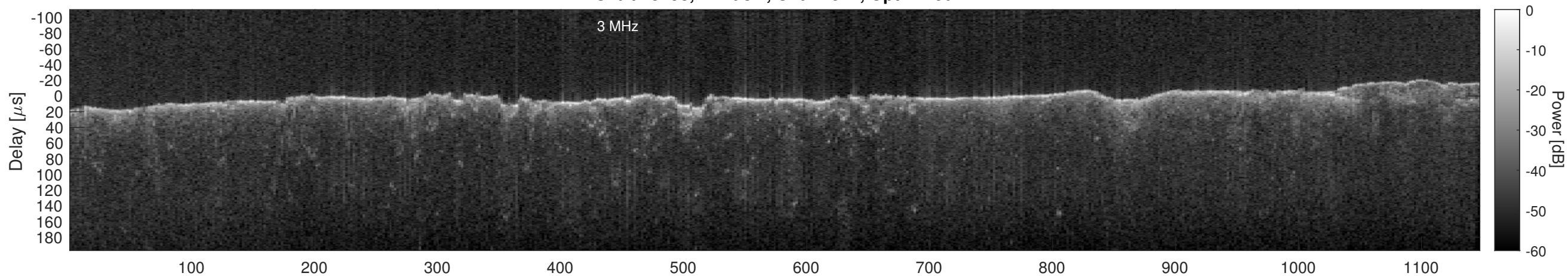
Orbit 15298, Cluttergram
