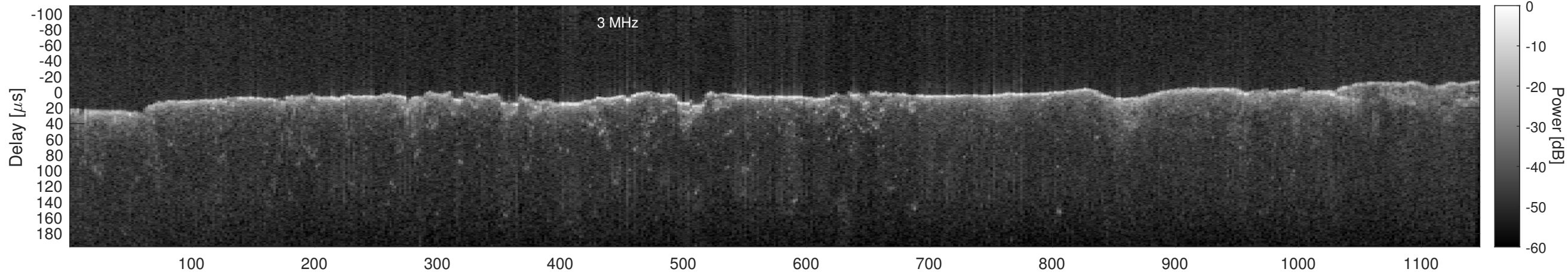
Orbit 15298, Window, Channel 2, Chapman
