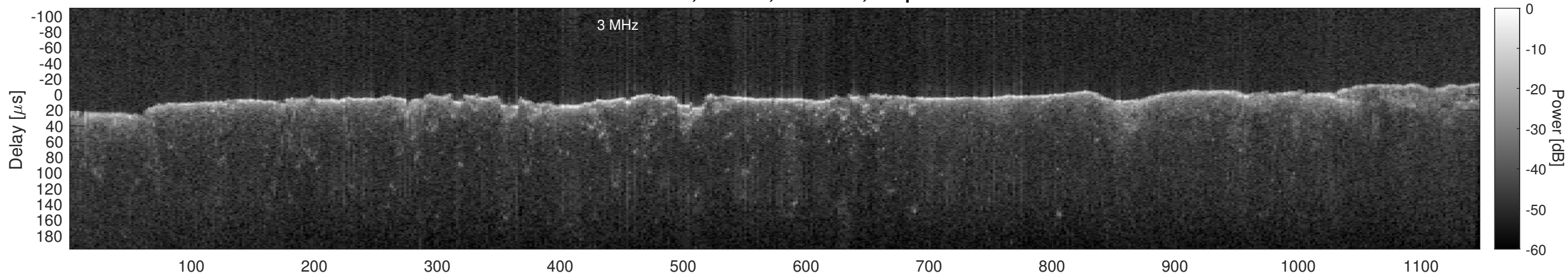
Orbit 15298, Window, Channel 2, Optimized
