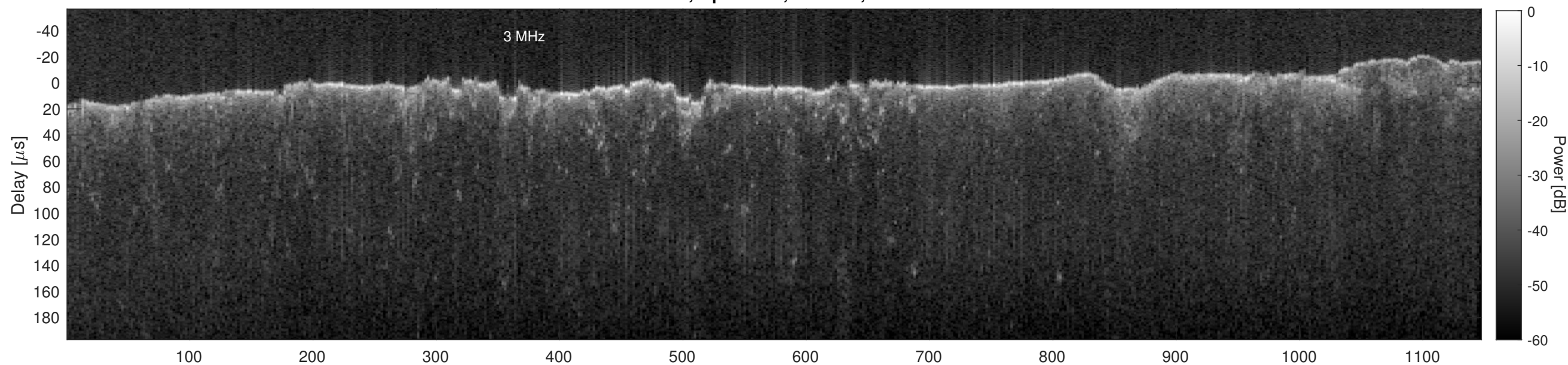
Orbit 15298, Cluttergram
