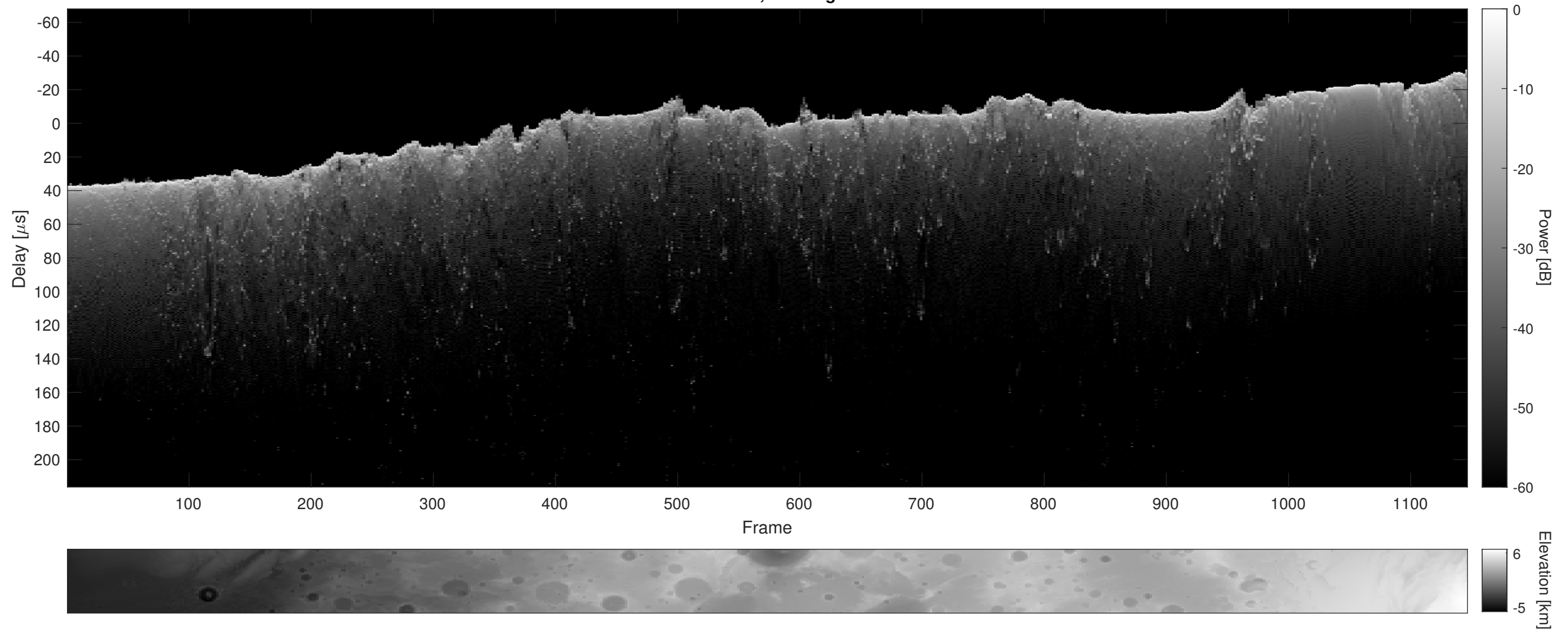
Orbit 15314, Cluttergram
