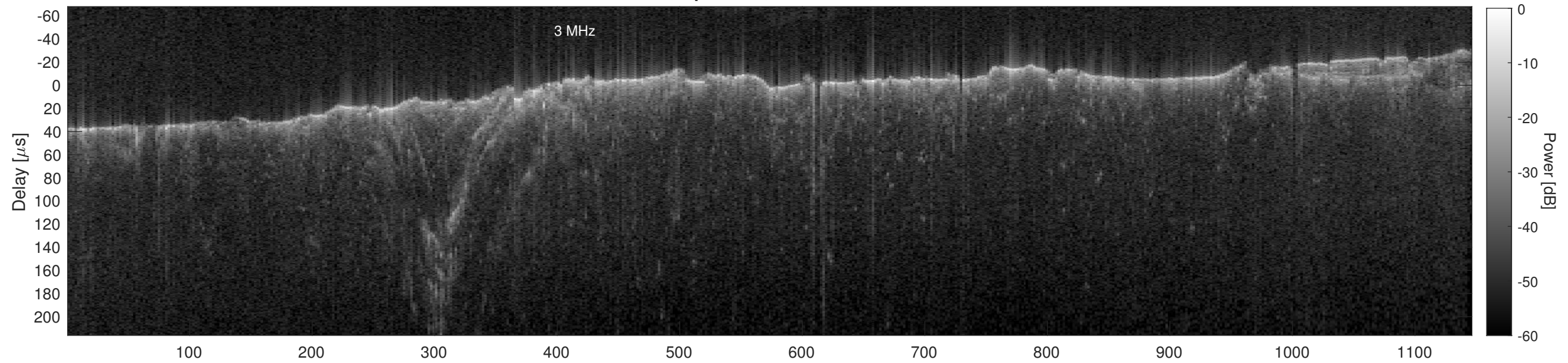
Orbit 15314, Cluttergram
