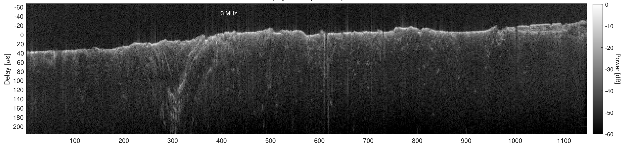
Orbit 15314, Cluttergram
