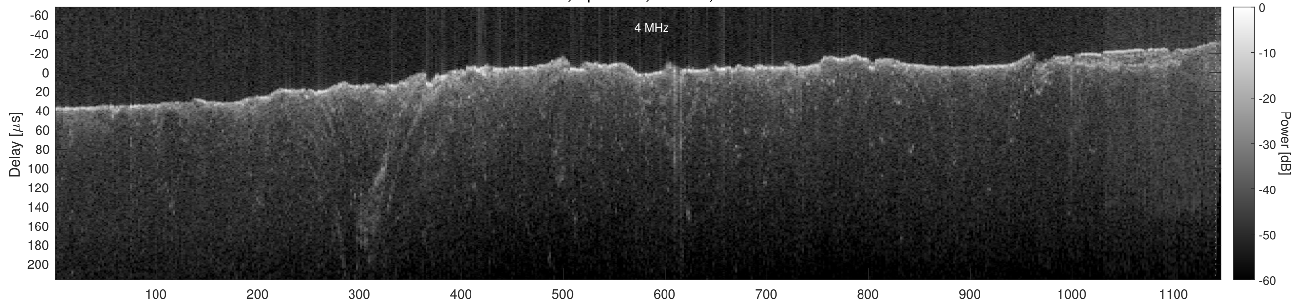
Orbit 15314, Optimized, Window, Channel 2
