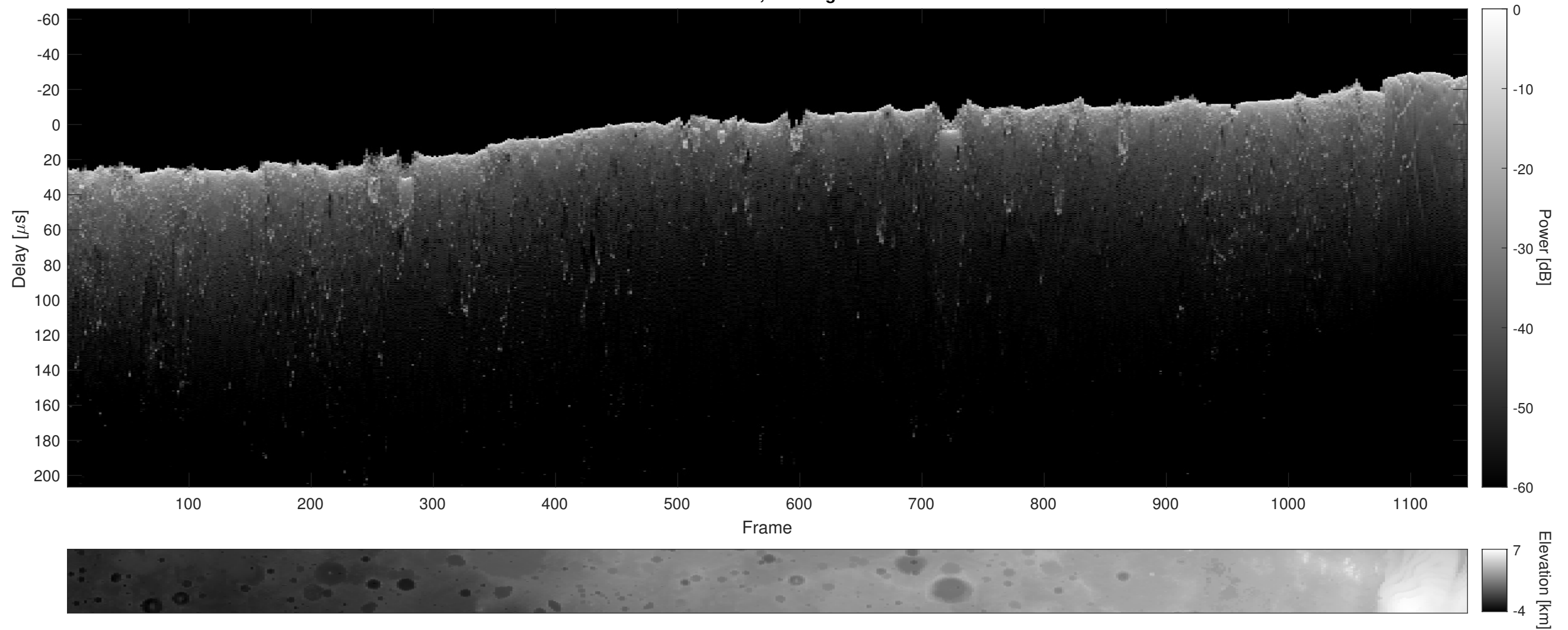
Orbit 15316, Cluttergram
