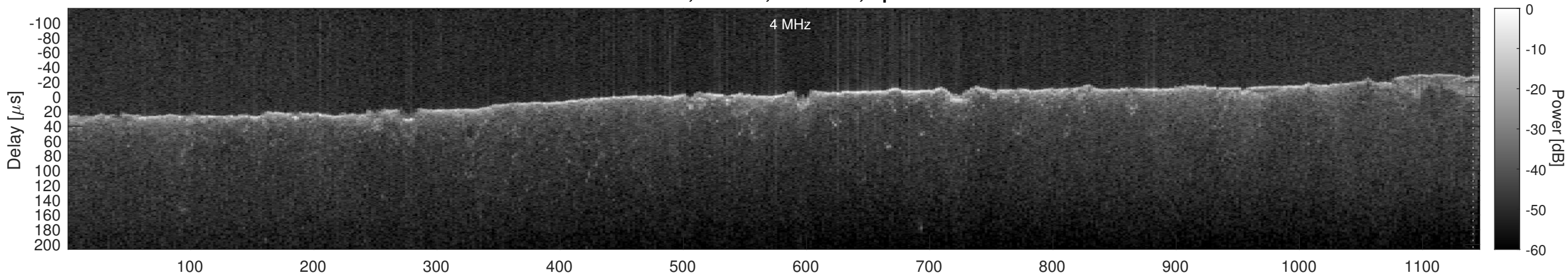
Orbit 15316, Cluttergram
