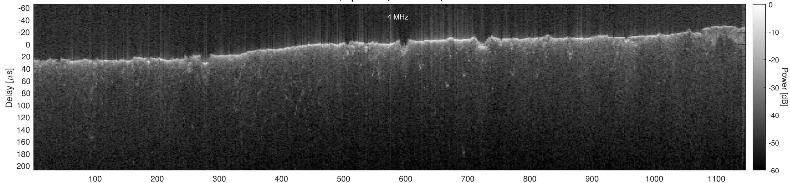
Orbit 15316, Optimized, No Window, Channel 2
