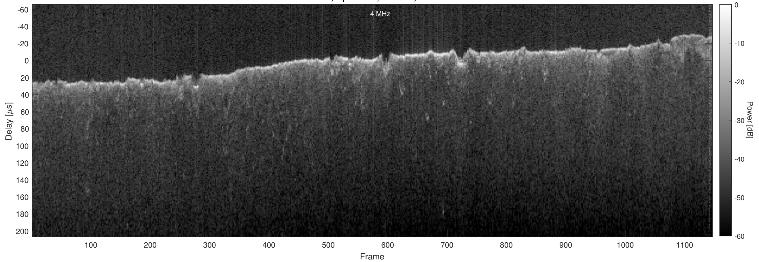
Orbit 15316, Optimized, Window, Channel 2
