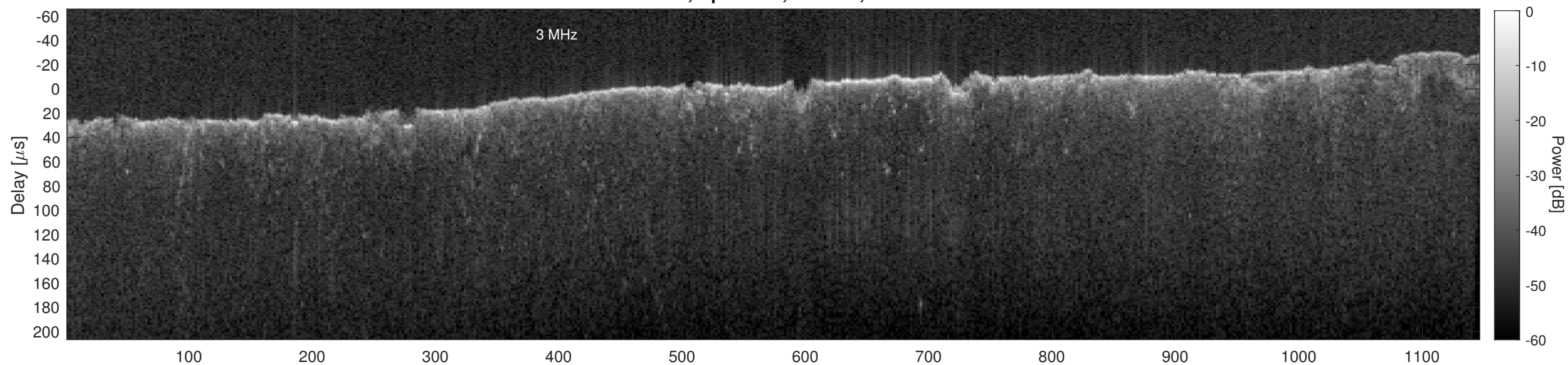
Orbit 15316, Cluttergram
