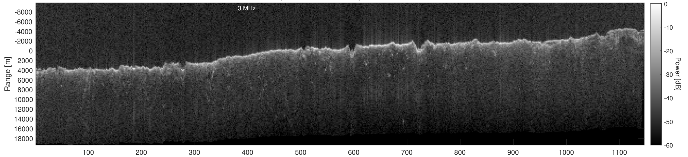
Orbit 15316, Depth-Corrected Cluttergram
