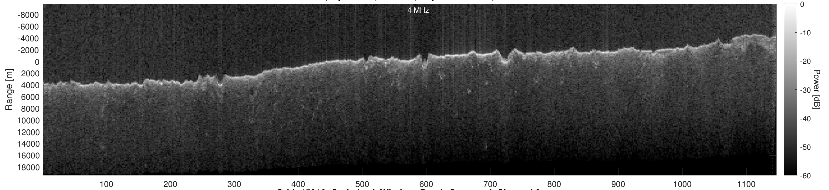
Orbit 15316, Optimized, Window, Depth-Corrected, Channel 2
