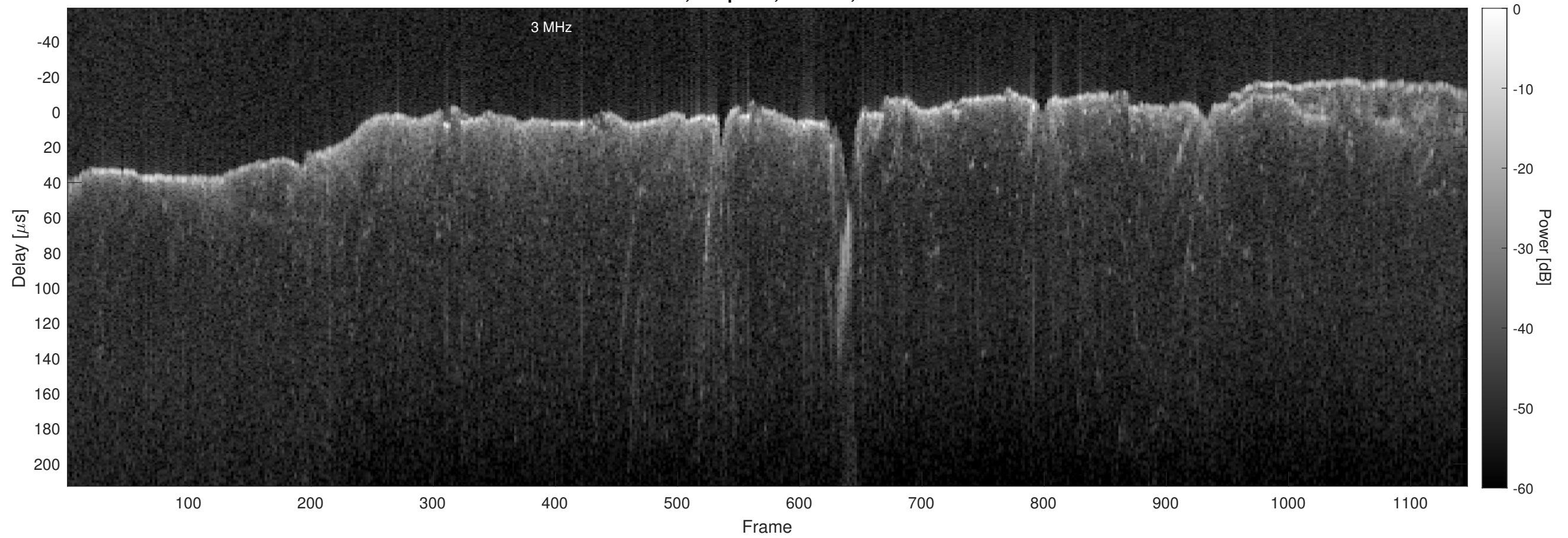
Orbit 15318, Chapman, Window, Channel 2
