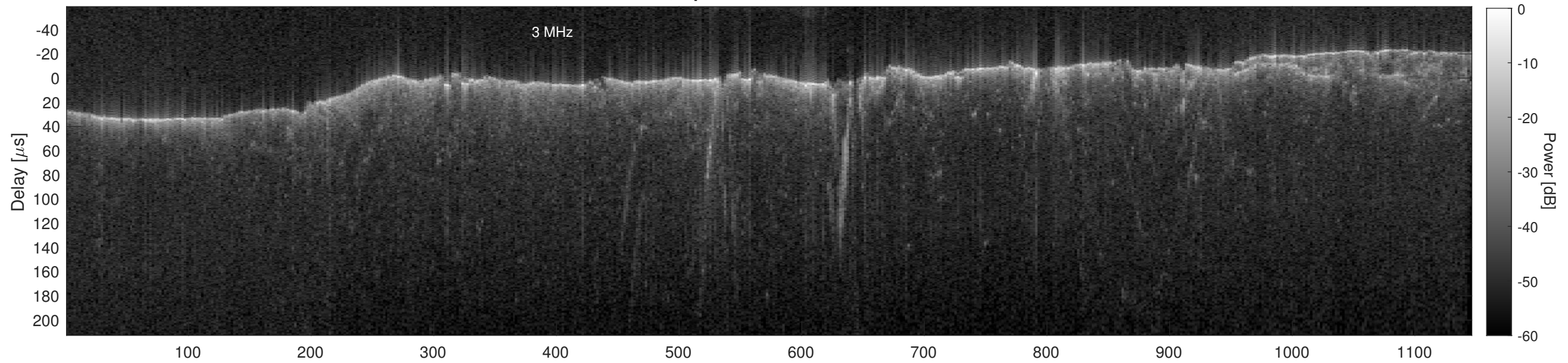
Orbit 15318, Cluttergram
