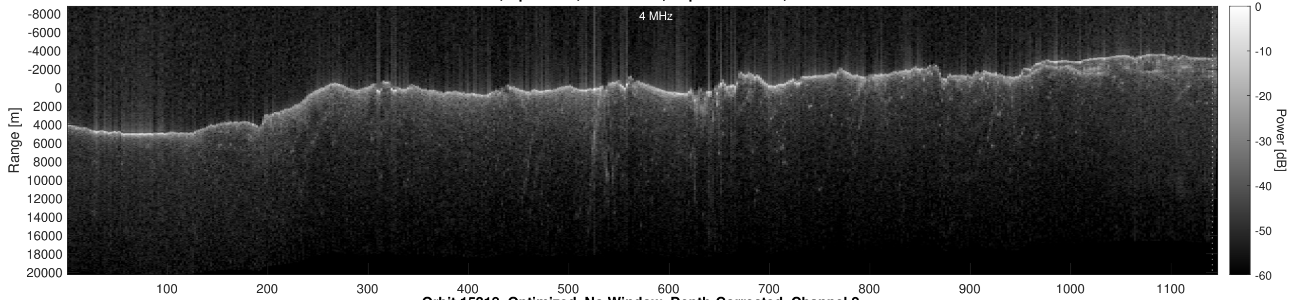
Orbit 15318, Optimized, No Window, Depth-Corrected, Channel 2
