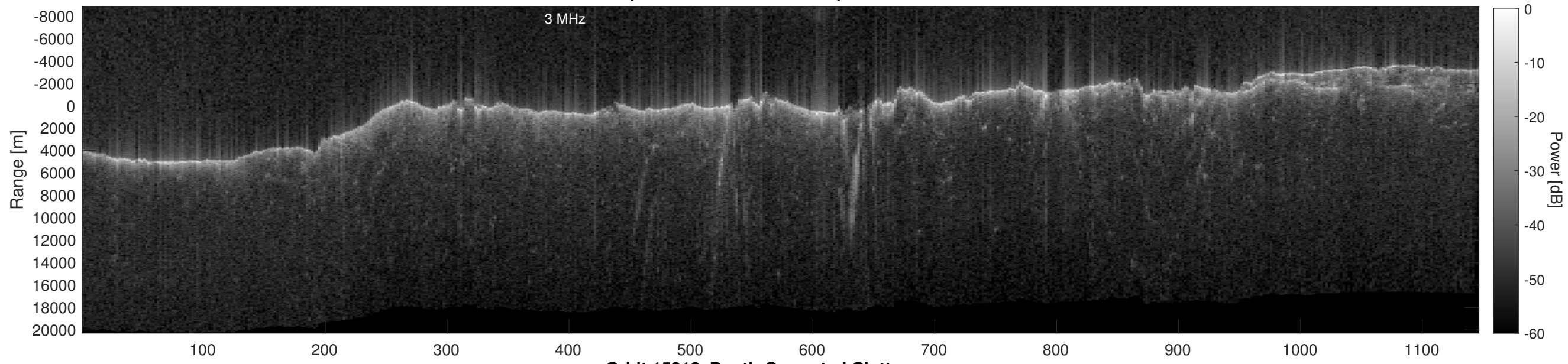
Orbit 15318, Depth-Corrected Cluttergram
