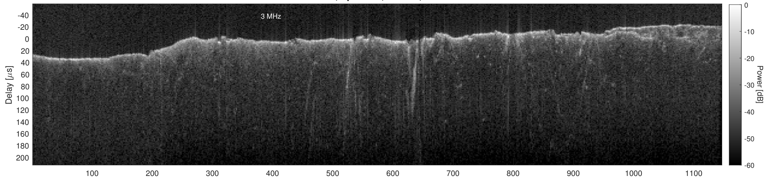
Orbit 15318, Cluttergram
