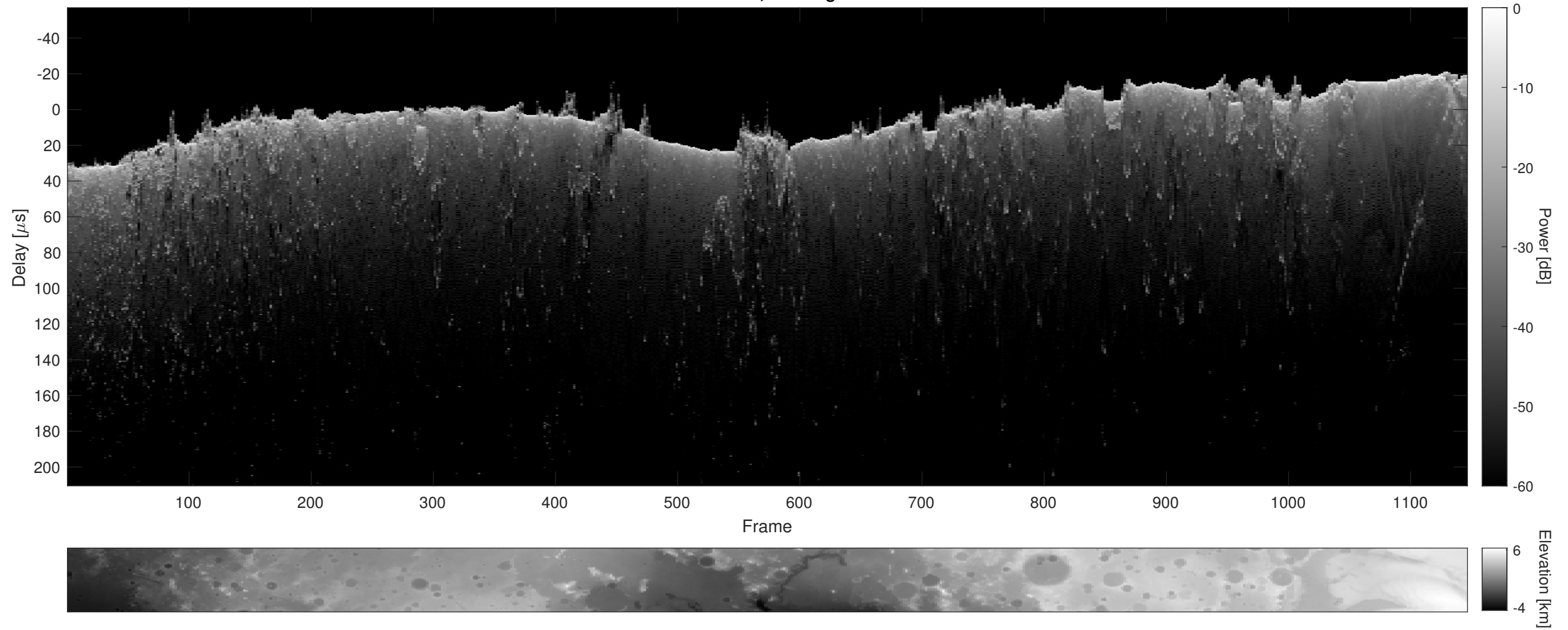
Orbit 15322, Cluttergram
