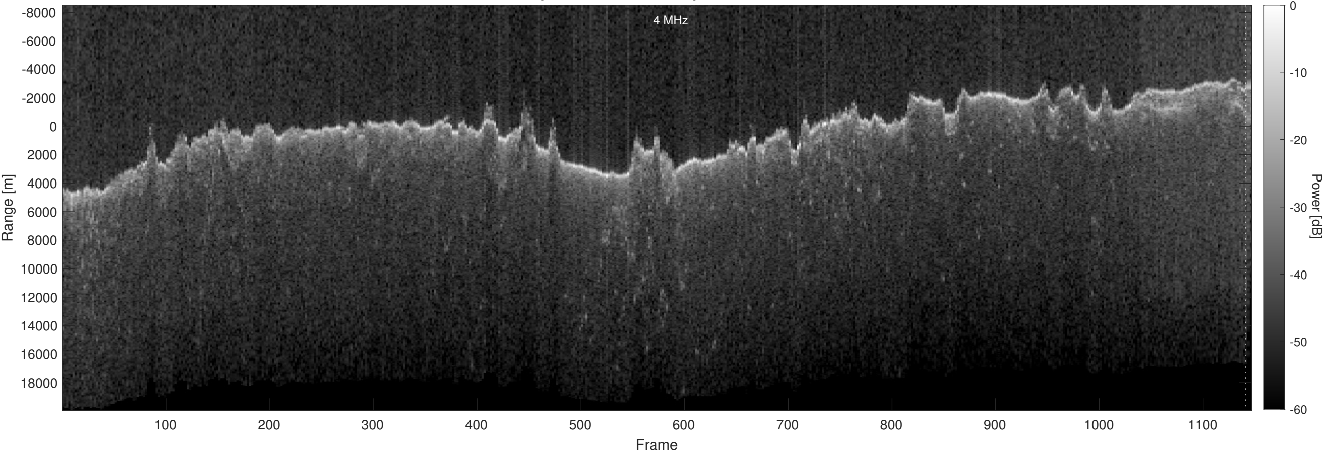
Orbit 15322, Optimized, Window, Depth-Corrected, Channel 2
