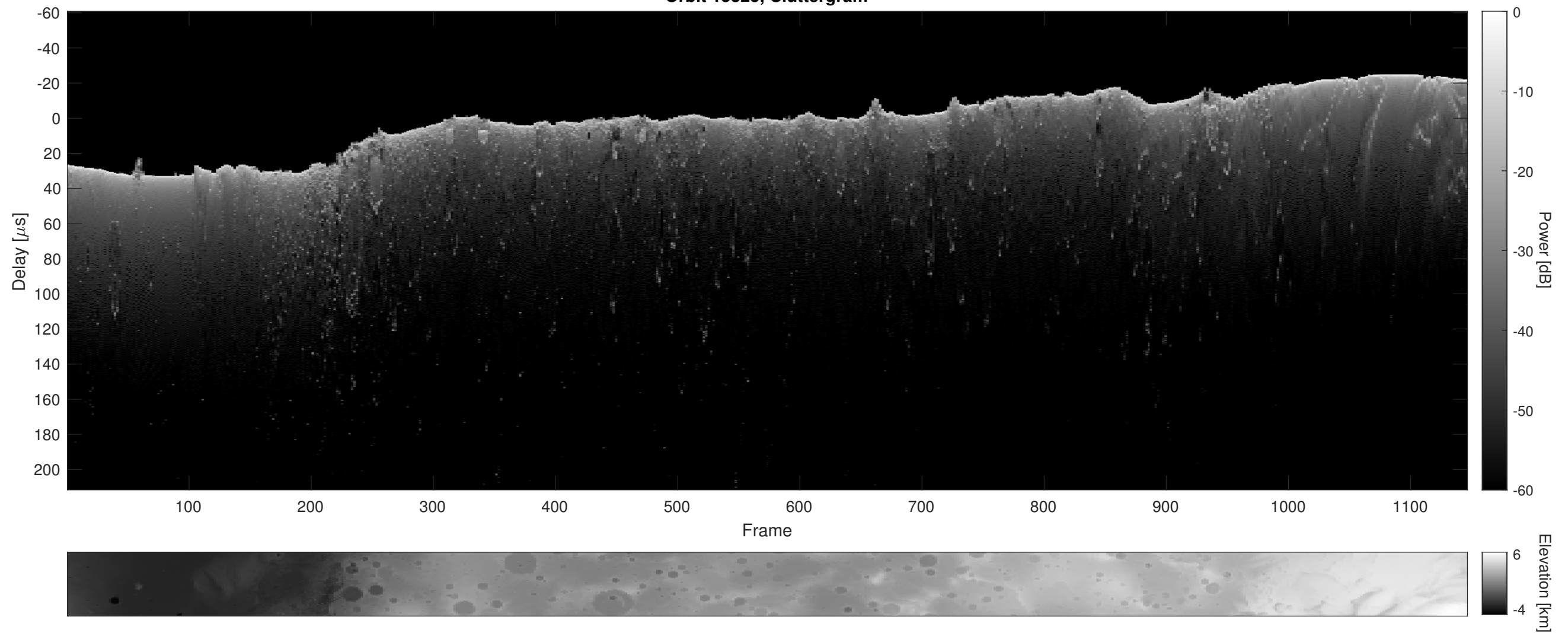
Orbit 15325, Cluttergram
