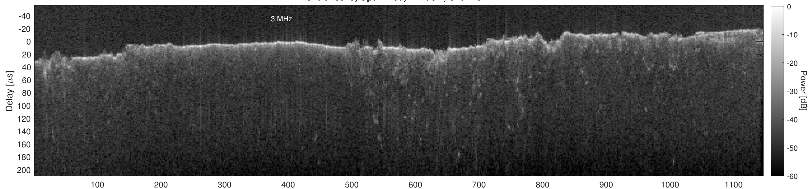
Orbit 15329, Cluttergram
