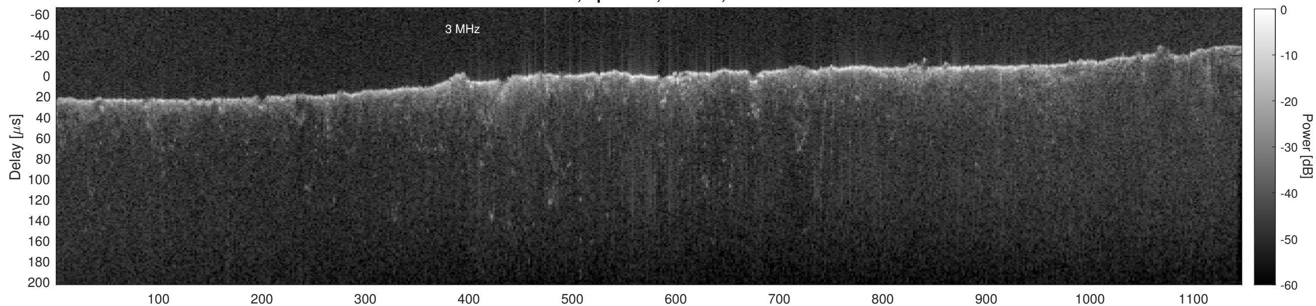
Orbit 15330, Cluttergram
