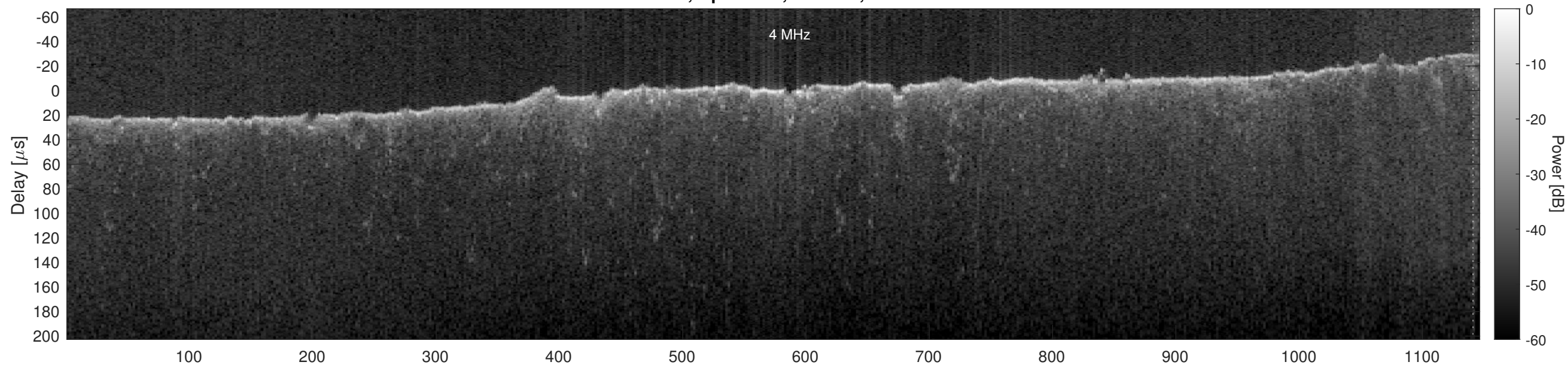
Orbit 15330, Optimized, Window, Channel 2
