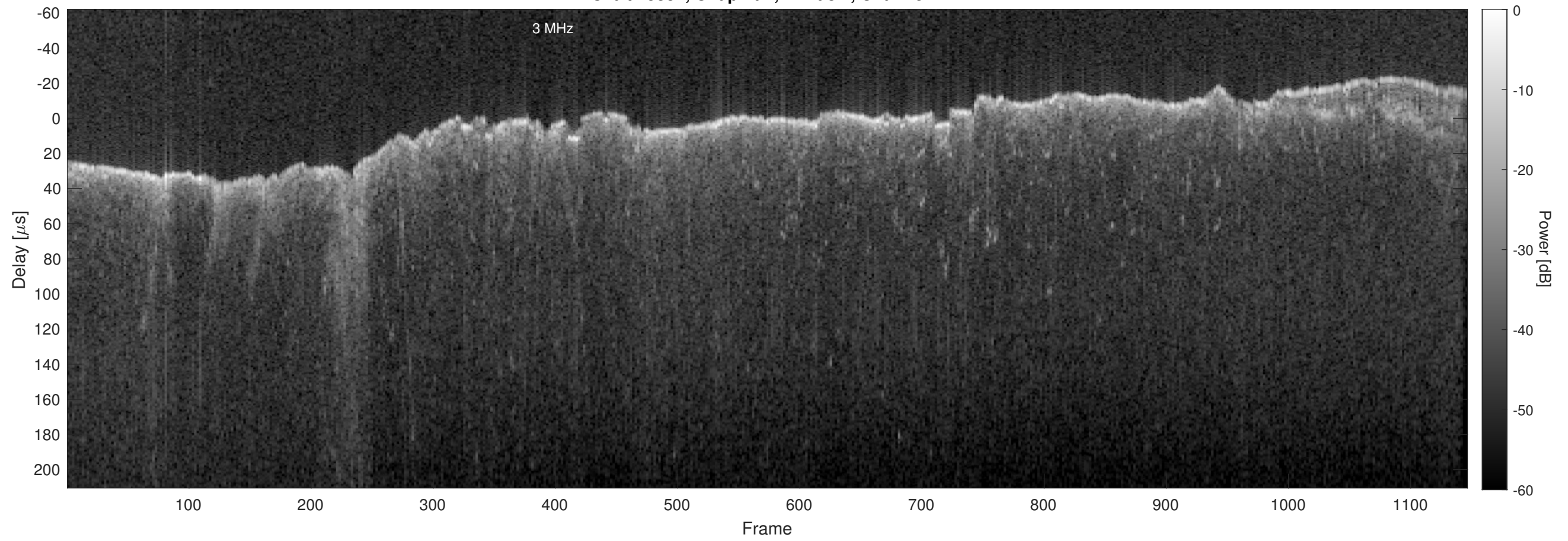
Orbit 15332, Chapman, Window, Channel 2
