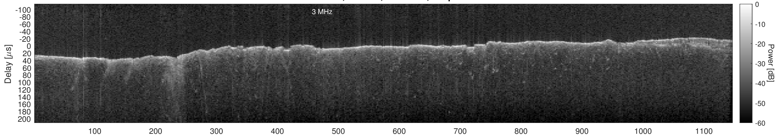
Orbit 15332, Window, Channel 2, Optimized
