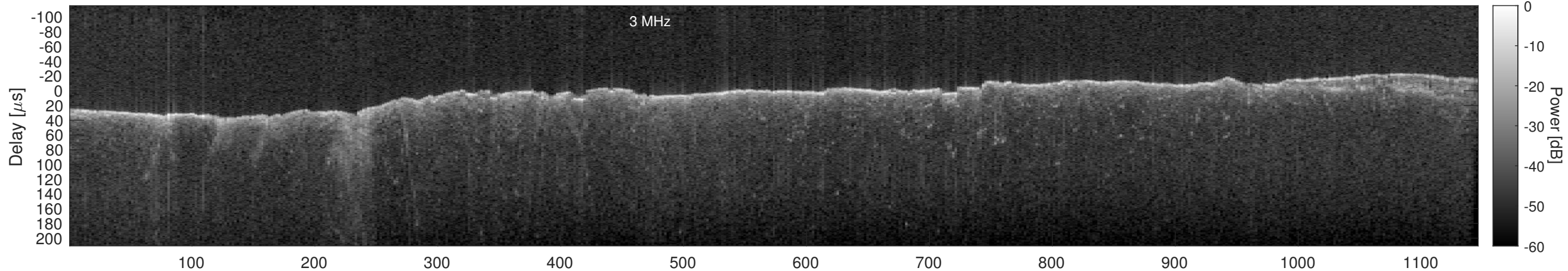
Orbit 15332, Window, Channel 2, Chapman
