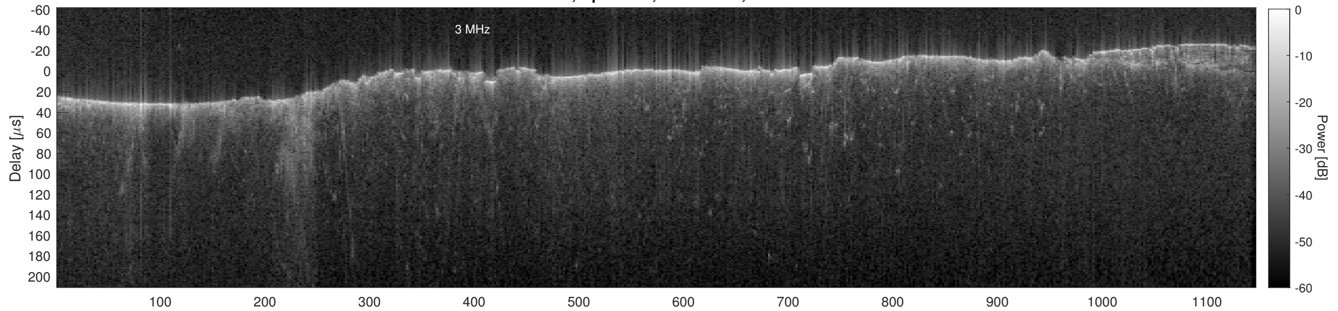
Orbit 15332, Cluttergram
