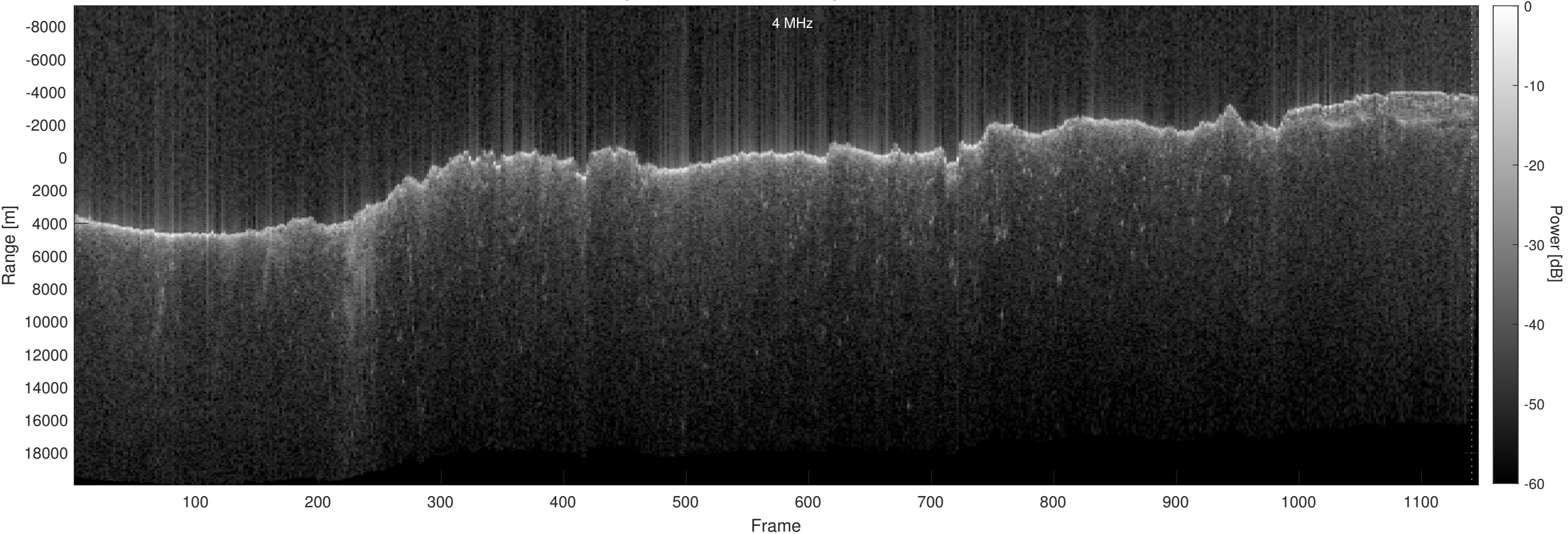
Orbit 15332, Optimized, No Window, Depth-Corrected, Channel 2
