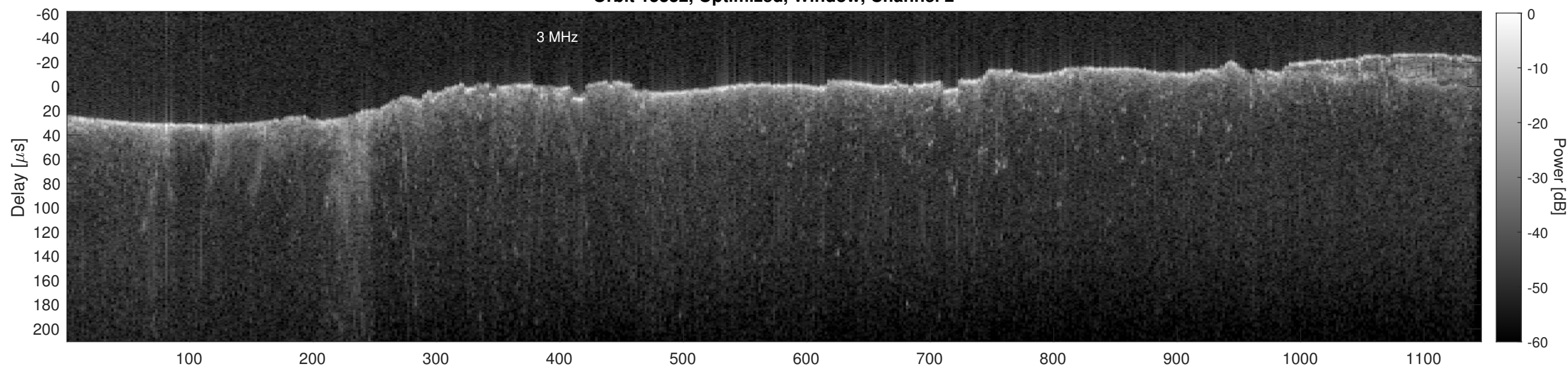
Orbit 15332, Cluttergram
